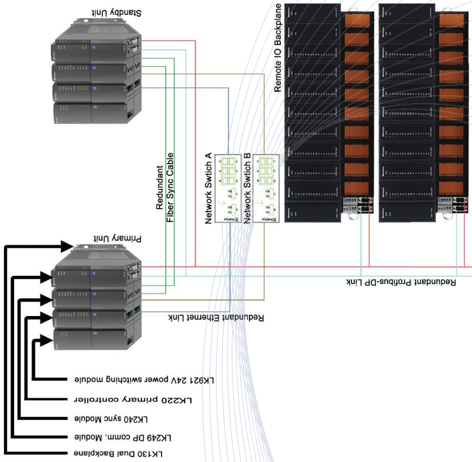
Figure 1.1 Network Connection of LK Master Controller
